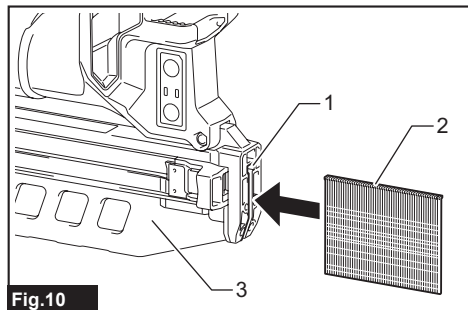
► 1. Slit 2. Fastener strip 3. Magazine
