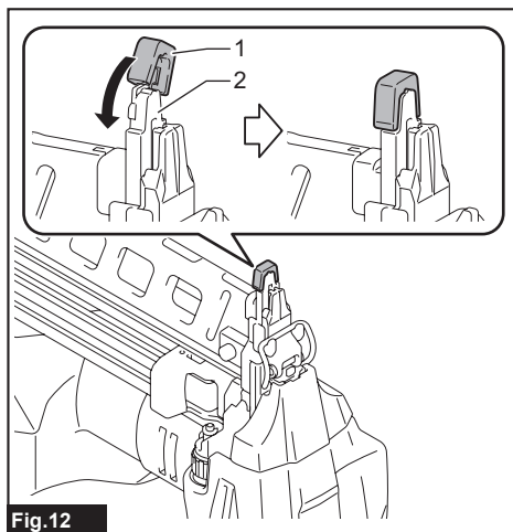
► 1. Nose adapter 2. Contact element
